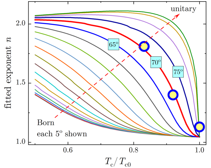
FIG. 4. Lines show the exponent n obtained from the power-law fitting up to T_c/3 , \rho_s(t) = 1 - Rt^n , of the superfluid density calculated numerically using the t -matrix theory. Different curves correspond to different values of the scattering potential strength, parameterized by the phase shift \theta . The disorder is presented via the reduced T_c(\Gamma)/T_{c0} , also accessible experimentally. Symbols show the exponents obtained from the experiment, also fitted up to T_c/3 . The best match is shown by a bold red line corresponding to \theta = 70^\circ .
