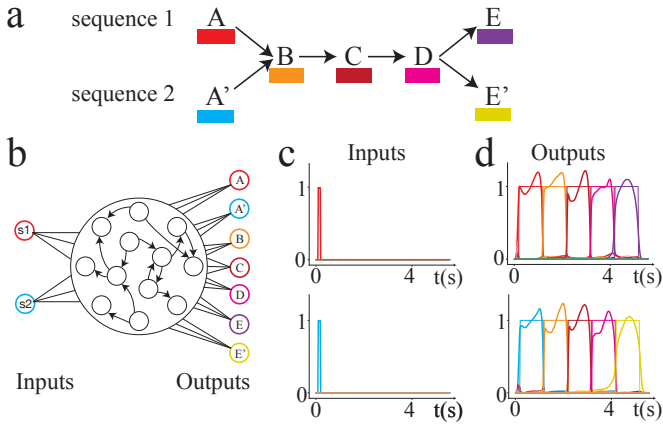
Fig. 1. a. Two sequences with long-distance-dependencies. For clarity, in subsequent figures each word is associated with a color, as in [4]. b. Cartoon of the trained neural architecture. c. One of two input neurons is transiently activated at the beginning of each sequence. d. Each of the output neuron is responsible for producing one of the 7 possible words of the sequence. Each colored line represents the activation of one of the readout neurons (thin lines represent the target activations, thick lines represent activations from trained networks).
