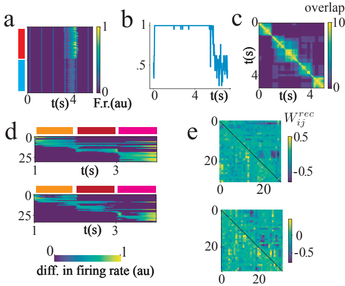
Fig. 3. a. Example of a neuron, connected to the readout D whose firing rate is modulated by the identity of the first red or blue word. b. Decoding performance of perceptrons trained to decode the first word from the firing rates of the 256 neurons at all times in the sequence. c. Cross-correlogram of decoding vectors: for each time point the perceptron is parametrized by a weight-vector, for each of these weight-vectors the 10 entries corresponding to the 10 neurons that participated the most in the first word prediction (highest absolute value) are set to 1, other entries to 0, to obtain the decoding vector. Color bar shows the scalar product between two decoding vectors obtained at different decoding time points. d. Rescaled differences in firing rates for the class A (top) and class A' (bottom) neurons. The color amplitude represents \log(1 + 100 * [fr1 - fr2]_+) with fr1 and fr2 the firing rates produced during sequence 1 and 2 and [\ ]_+ the sign rectification function. e. Connectivity matrix of the class A (top) and A' (bottom) neurons. Neurons are ordered according to their time of maximal firing rate modulation.
