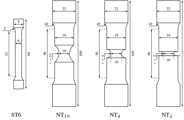
Figure 2: Geometries of the smooth tensile specimen ST6, Notch tensile specimens NT 2 , NT 4 and NT 10 (unit: mm).
