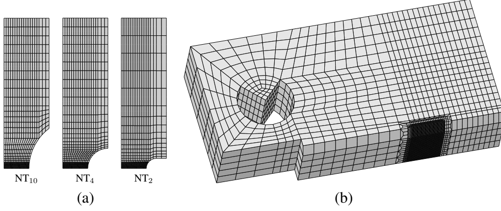
Figure 13: Meshes for (a) NT 2 , NT 4 , NT 10 and (b) C(T)20 specimens.
