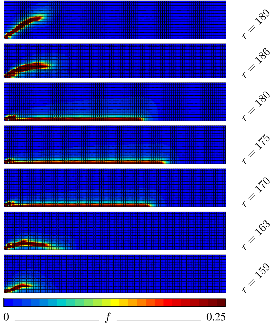
Figure 20: Distribution of porosity f along the circumferential direction for different radii r (mm) when CMOD= 9.6 mm (values at integration points). Plots in the undeformed initial configuration.
