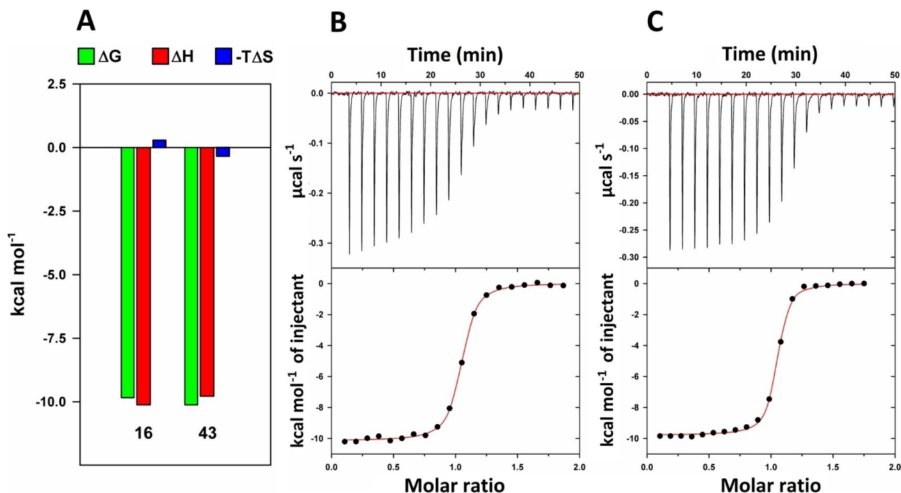
Figure 2. (A) VIM-2 binding energetics of compound 16 and 43 . Data are from Table 2. (B) and (C) Isothermal titration calorimetry of VIM-2 by compounds 16 and 43 at 25 °C. Upper panel: exothermic microcalorimetric trace of compound injections into VIM-2 solution (18.7 \mu\text{M} ). Lower panel: Wiseman plot of heat releases versus molar ratio of injectant/protein in the cell and nonlinear fit of the binding isotherm for n equivalent binding sites. The binding enthalpy corresponds to the amplitude of the transition curve, K_d is derived from the slope of the transition and the stoichiometry n is determined at the transition midpoint.
