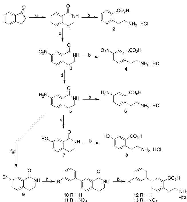
Scheme 2. Synthesis of the 2-(2-aminoethyl)benzoic acids precursors R^2\text{-NH}_2 2 , 4 , 6 , 8 , 12 , 13 . Reagents and conditions: (a) Conc. HCl, \text{NaN}_3 , rt, 15 h; (b) Conc. HCl, 110 °C, 15 h; (c) Fuming \text{HNO}_3 , \text{H}_2\text{SO}_4 , 0 °C, 1 h30; (d) \text{H}_2 , 10% Pd/C, rt, 8 h; (e) \text{H}_2\text{SO}_4 , \text{NaNO}_2 , water, 0 °C, 40 min, +90 °C, 1 h30; (f) 48% HBr, \text{NaNO}_2 , water, 0 °C, 30 min; (g) CuBr, rt, 30 min +70 °C, 1 h; (h) phenylboronic acid or 3-nitro-phenylboronic acid, 2 M aq. \text{Na}_2\text{CO}_3 , toluene/MeOH, tetrakis, reflux, 4 h.
