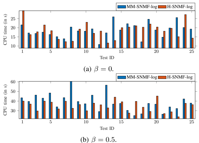
Fig. 6: Comparative performance with a spectrogram using the log-regularization.
