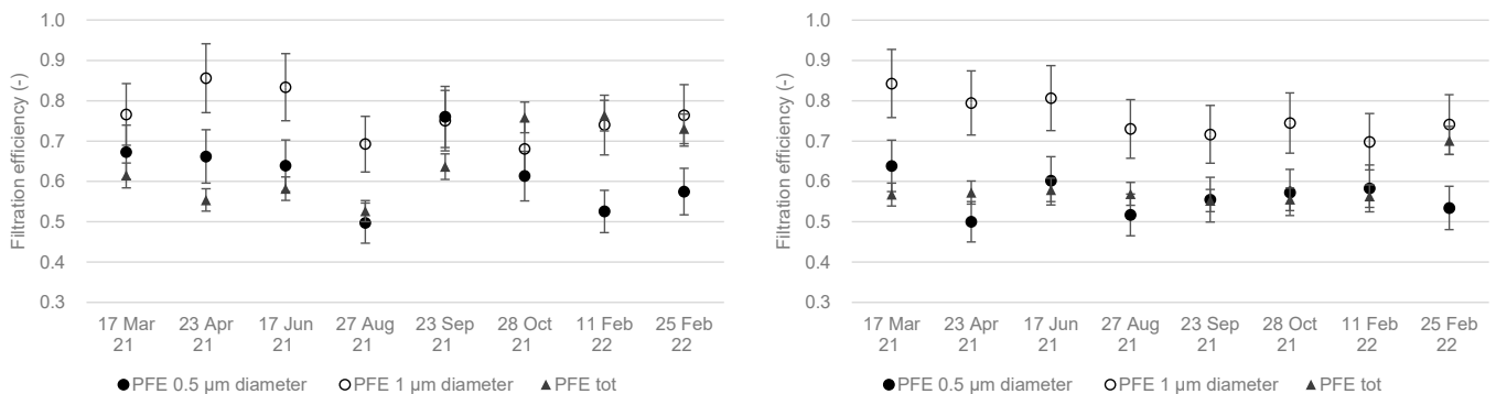
Figure 7. Total particle filtration efficiency and filtration efficiency for aerosol diameters 0.5 \mu\text{m} and 1 \mu\text{m} in the fresh air (left) and extracted air (right) compartments over 12 months.
