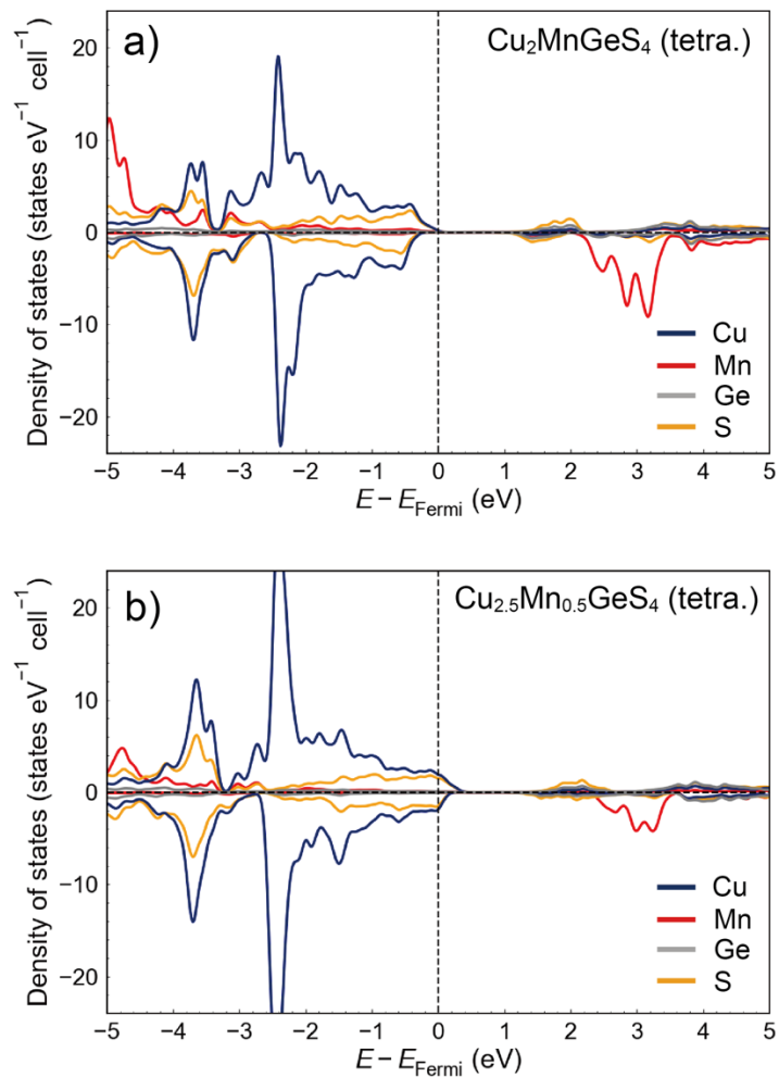
Figure S10. Element-deconvoluted electronic density of states (DOS) of (a) tetragonal \text{Cu}_2\text{MnGeS}_4 and (b) \text{Cu}_{2.5}\text{Mn}_{0.5}\text{GeS}_4 . E_{\text{Fermi}} is the Fermi energy. Positive and negative DOS indicate the partial DOS of up-spin and down-spin orbitals, respectively.
