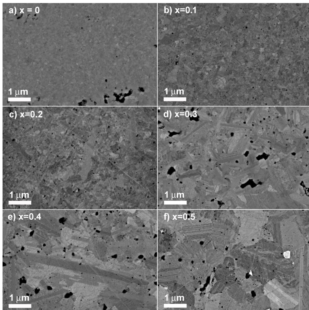
Figure 7. SEM micrographs of polished surfaces in the \text{Cu}_{2+x}\text{Mn}_{1-x}\text{GeS}_4 series.
