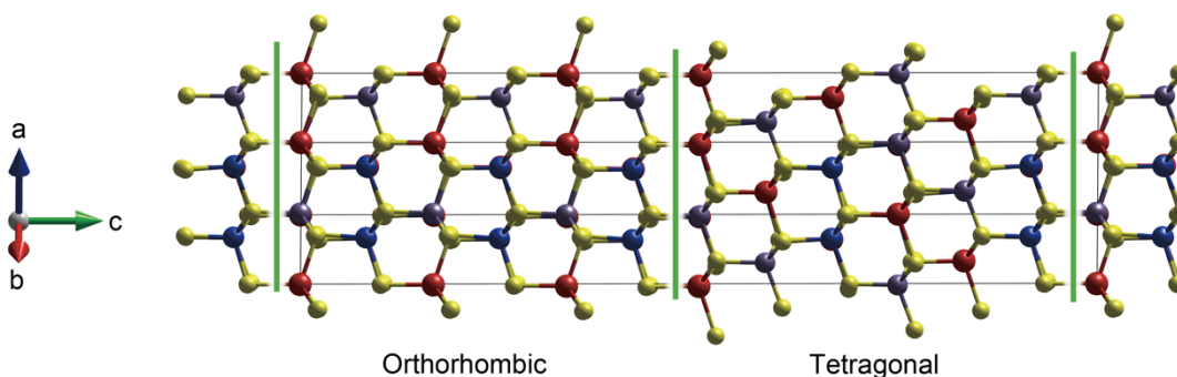
Figure 8. Fully relaxed structures of two phases with interfaces. (a) Stacking faults in the orthorhombic enargite-type phase, (b) twin boundaries in the tetragonal stannite-type phase and (c) coherent interfaces between the orthorhombic enargite-type and tetragonal stannite-type phases. Blue, red, gray, and yellow balls indicate \text{Cu}^+ , \text{Mn}^{2+} , \text{Ge}^{4+} and \text{S}^{2-} ions, respectively. The cell dimensions of these interface models are (a) a = 7.698 \text{ \AA} , b = 6.560 \text{ \AA} , c = 37.640 \text{ \AA} ; (b) a = 7.730 \text{ \AA} , b = 6.550 \text{ \AA} , c = 37.491 \text{ \AA} ; (c) a = 7.715 \text{ \AA} , b = 6.554 \text{ \AA} , c = 37.569 \text{ \AA} . Green lines are eye guides for viewing the positions of these planer defects. These structures are drawn using VESTA. [35]
