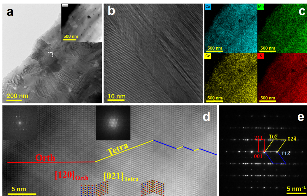
Figure 3. Microstructure characterization of \text{Cu}_{2.3}\text{Mn}_{0.7}\text{GeS}_4 sample. (a, b) TEM images. (c) EDX mapping of the corresponded area in the inset HAADF image of (a), HAADF image (d) and (e) the corresponding SAED pattern of \text{Cu}_{2.3}\text{Mn}_{0.7}\text{GeS}_4 .
