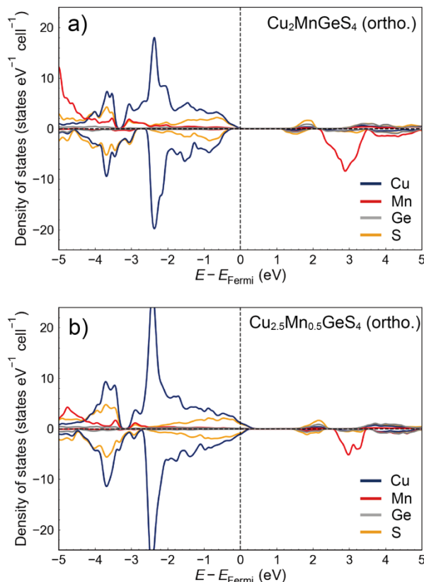
Figure 10. Element-deconvoluted electronic density of states (DOS) of (a) orthorhombic enargite-type \text{Cu}_2\text{MnGeS}_4 and (b) \text{Cu}_{2.5}\text{Mn}_{0.5}\text{GeS}_4 phases. E_{\text{Fermi}} indicates the Fermi energy. Positive and negative DOS indicate the partial DOS of up-spin and down-spin orbitals, respectively.
