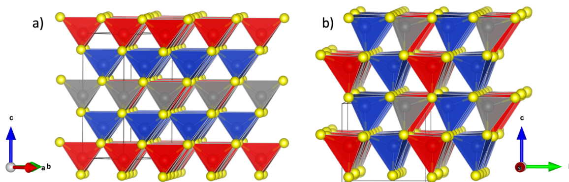
Figure 1. Crystal structure representation of \text{Cu}_2\text{MGeS}_4 phases with a) a tetragonal stannite-type structure ( M = \text{Fe, Co, Hg} ) and b) an orthorhombic enargite-type structure ( M = \text{Mn, Ni, Zn, Cd} ). Key: copper in blue; M in red; Ge in grey; sulfur in yellow.
