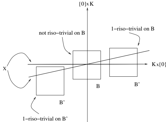
FIGURE 2. Applying Theorem 2.8 in Example 2.13
