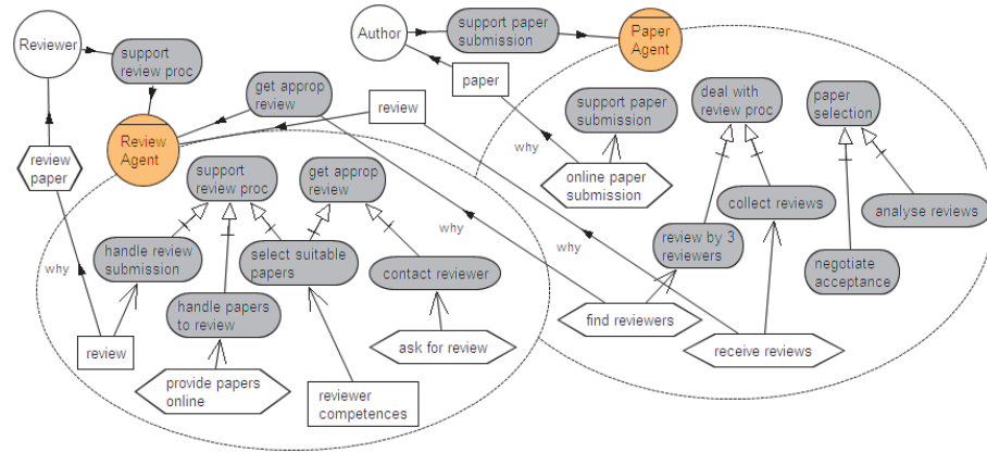
Fig. 7. Details from the goal models of the sub-actors paper and reviewer. Key in Fig. 6.
