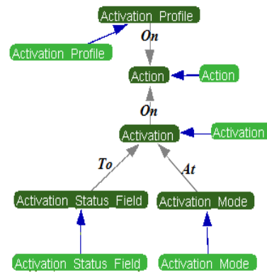
Figure 2: Functional relations established between ConceptAgents
