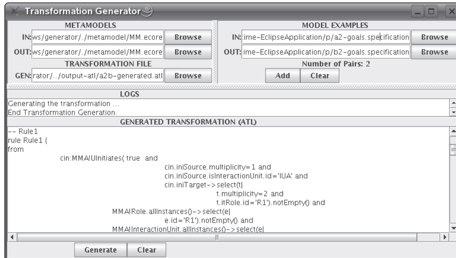
Fig. 2. Model-Transformation Generator Tool
