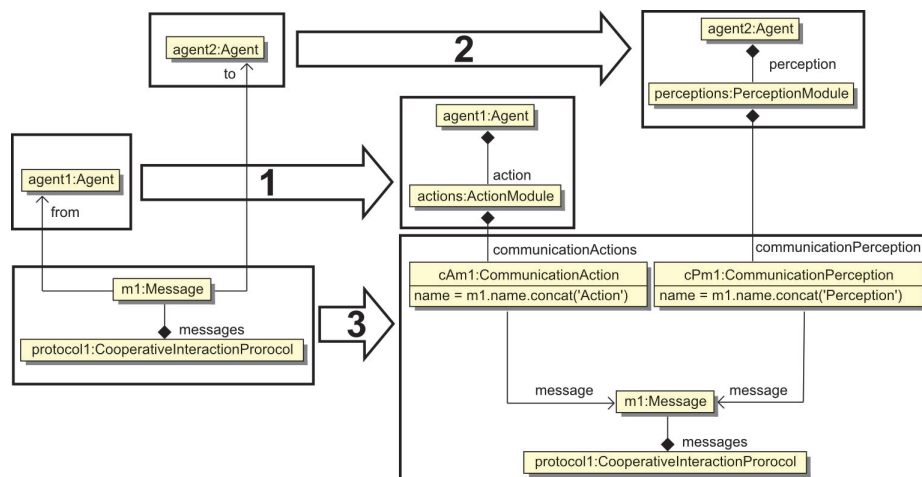
Fig. 4. Model refactoring example in ADELFE using MTBE : creating communication action and perception in respective modules for each message specified in AMAS-ML interaction protocols
