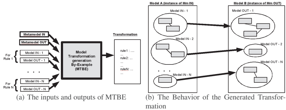
Fig. 1. Description of the Model Transformation By-Example (MTBE)
