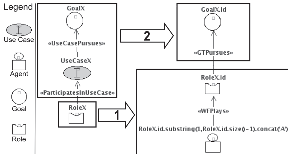
Fig. 3. Model transformations for generating the Specification of Roles. Each square represent a model example for MTBE. Each pair of models is related with an arrow and a number, in which the source and target models are respectively situated at the left and right sides of the arrow.
