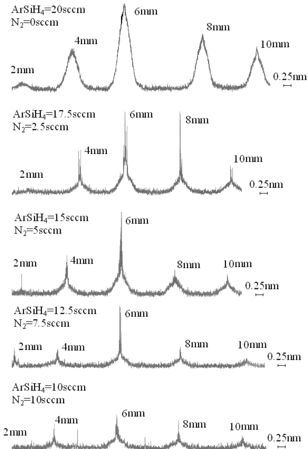
FIG.4. Comparison of the H \alpha Balmer line measured in different positions from 2mm to 10mm above the cathode along the discharge axis and for different gas mixtures, the total gas flow rate is of 20sccm and the total pressure of 0.53mbar.
