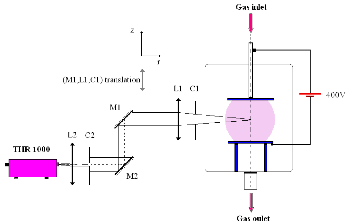
FIG.1. Experimental setup.
