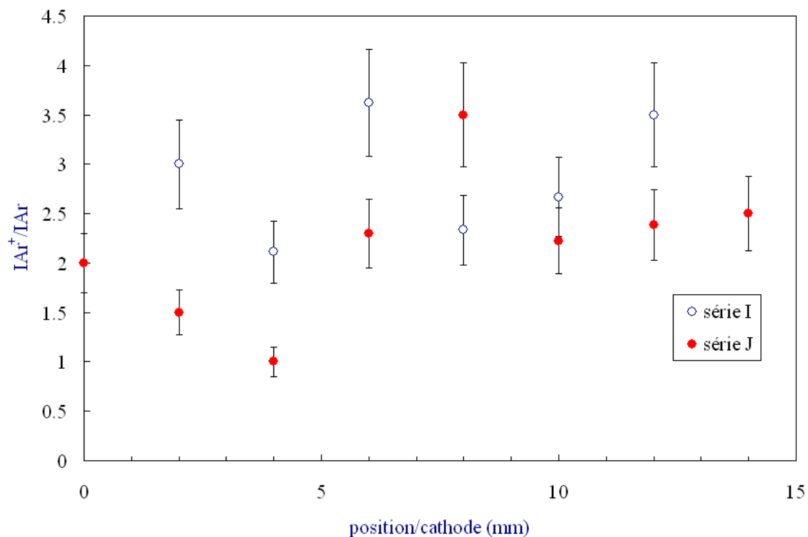
FIG.7. Relative intensity of I_{ArII}(413.1nm)/I_{ArI}(419.1nm) versus distance from the cathode along the inter electrode axis in pure argon (series I) and in Ar\text{-}\%SiH_4 (series J), at 400V, 13mA and 0.53mbar.
