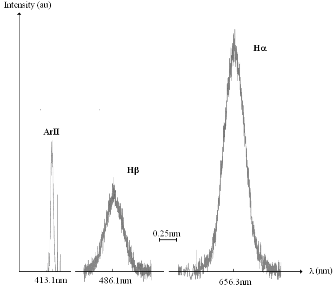
FIG.2. Emission lines measured for ArII(413.1nm), Hα (656.3nm) and Hβ (486.1nm); Comparison of the emission line widths.
