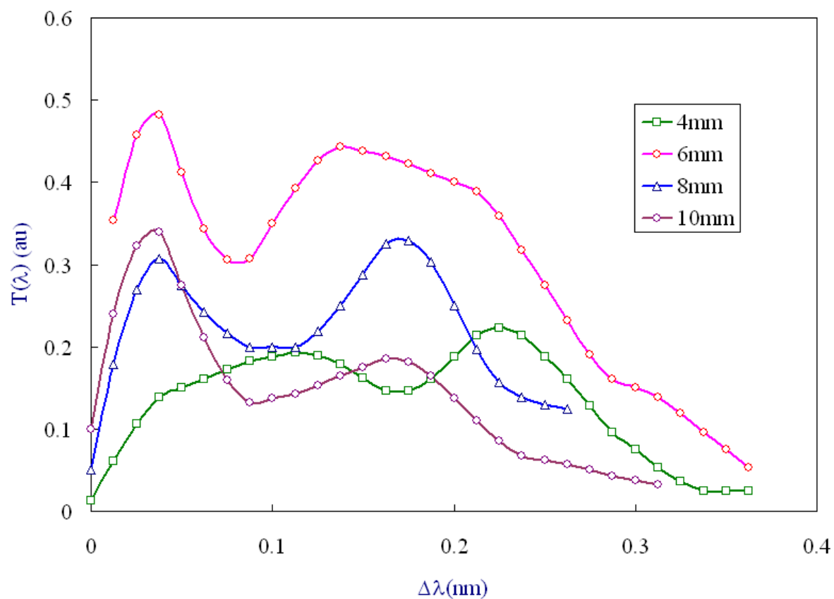
FIG.6. Translational energy distribution of H atoms measured on H\alpha in Ar-SiH 4 discharge at 0.53mbar in different positions from the cathode surface. Observations are performed perpendicularly to the inter electrode discharge axis.
