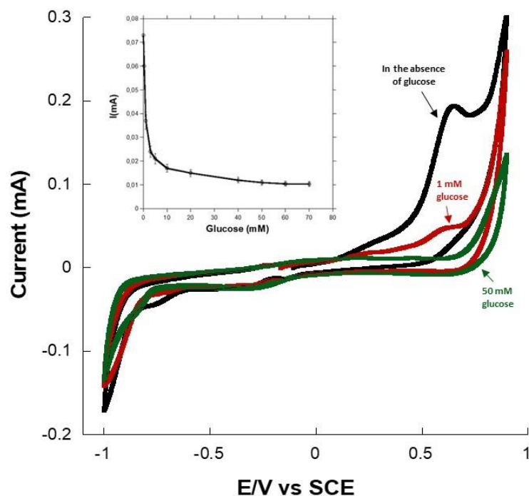
Figure 6. Cyclic voltammograms of the gold-PMG-ALDR-NADPH electrode at 2 \text{ mV} \cdot \text{s}^{-1} examined in pH 7 PBS in the absence and the presence of 1- and 50-mM glucose. Inset, oxidation current at +0.62 V as a function of glucose concentration (3 repetitions).
