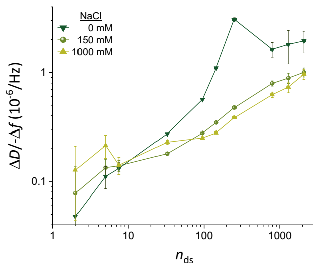
Figure 5. Effect of ionic strength on \Delta D/\Delta f ratios. Double logarithmic plot of \Delta D/\Delta f ( i=3 ; frequency shifts are normalised by i ) as a function of the mean number of disaccharides ( n_{ds} ) per HA chain, for NaCl concentrations of 0 mM, 150 mM and 1000 mM (as indicated with symbol and colour code). Representative data for one experiment per HA size are shown. The mean values represent the \Delta D/\Delta f ratio measured at high GAG surface densities (i.e., the maximal surface densities that were attained in the experiments and stable at 0 mM NaCl; see Fig. S2 for original data). The error bars account for baseline drifts during GAG binding. In the cases of 0 and 1000 mM NaCl, solution effects on the QCM-D response (i.e., owing to the effect of salt on solution density and/or viscosity) needed to be corrected for with the aid of control data, and uncertainties associated with this correction are also included in the error bars (see Fig. 1c and Supplementary Methods for details).
