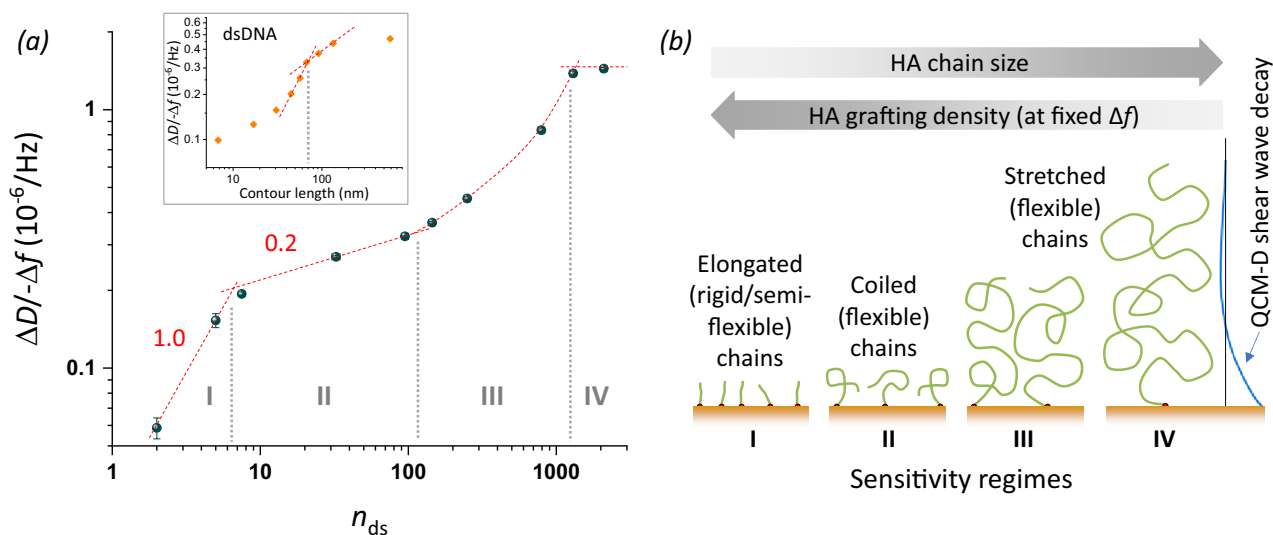
Figure 8. Sensitivity regimes of HA and underpinning mechanisms. (a) Double-logarithmic plot of the \Delta D/-\Delta f ratio ( i=3 ) at low HA surface density ( -\Delta f=2.5 Hz) as a function of the mean number of disaccharides, n_{ds} . Data for HA (blue spheres with error bars) are reproduced from Fig. 4. Sensitivity regimes I–IV are separated by vertical grey dotted lines. Regimes I and II are discerned by their distinct power-law dependencies (red dashed lines with slope illustrate the approximate power); regime III does not obey a power law (red curved dashed line illustrates the trend) and regime IV is close to a plateau/maximum (indicated by a horizontal line). The inset shows equivalent data for dsDNA extracted from Fig. 3 of Ref. 46 , with two selected power law dependencies (dashed red lines). (b) Illustration of the proposed model to explain the observed sensitivity regimes. Both HA chain size and grafting density (which decreases with increasing chain size at the set -\Delta f=2.5 Hz) influence chain conformation, and distinct chain conformations are associated with sensitivity regimes I, II and III; ultimately, chain stretching exceeds the QCM-D sensing depth leading to a \Delta D/-\Delta f maximum and vanishing size sensitivity in regime IV.
