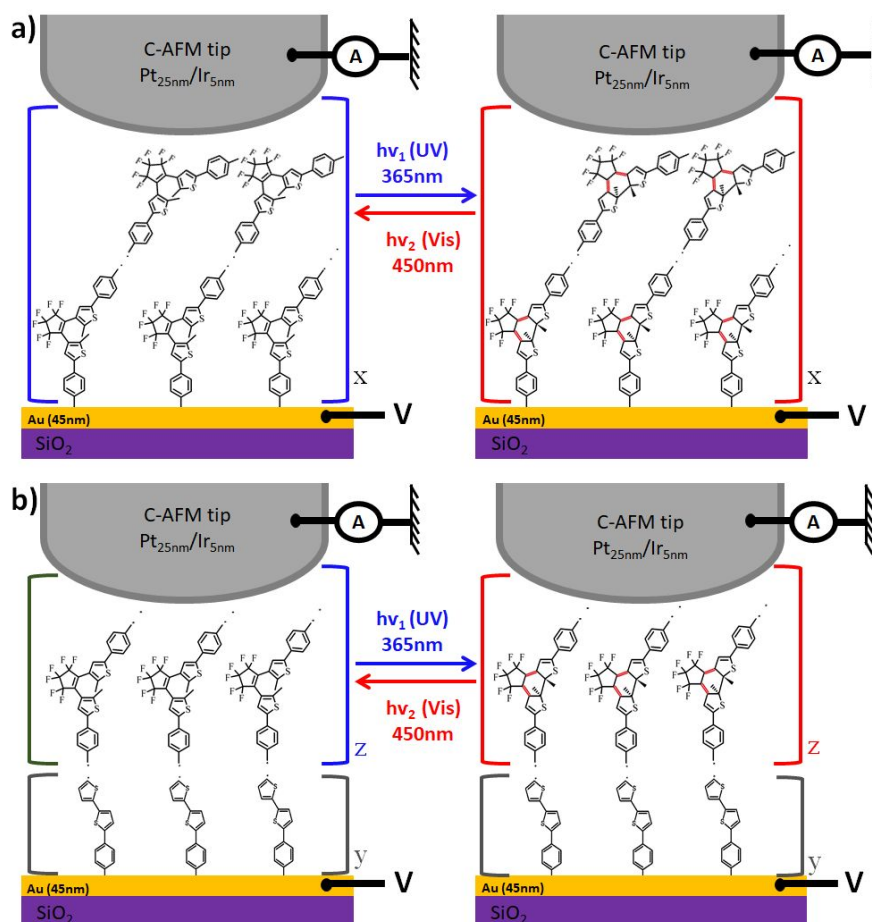
Figure 4. Schematic illustration of (a) SiO 2 /Ti 2nm /Au 45nm /oligo(DAE) 8-9nm /CAFAM tip (Pt 25nm /Ir 5nm ) (b) SiO 2 /Ti 2nm /Au 45nm /oligo(BTB) 4-5nm /oligo(DAE) 4nm /CAFAM tip (Pt 25nm /Ir 5nm ) molecular junction. x,y,z are numbers of repeating units of the oligomers which determine the thickness of the layer. The switch of the DAE units is turned ON by UV and OFF by visible light.
