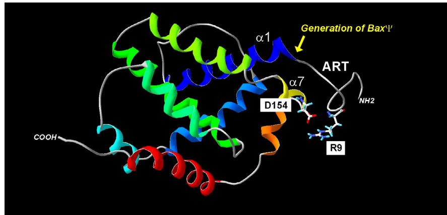
Figure 2. Regulation of Bax mitochondria localization by the ART. The absence of the ART (20 N-terminal residues) generates the Bax \Psi variant, which is spontaneously mitochondrial and active. Within the ART, the R9 residue may interact with the residue D154 of helix \alpha 7 . Point mutations in the helix \alpha 1 decrease the mitochondrial localization of both wild-type Bax (BaxWT) and Bax \Psi . Together, these data suggest that a movement of ART away from the core of the protein may contribute to the exposure of helix \alpha 1 to mitochondrial partners
