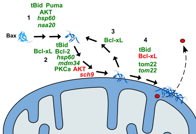
Figure 1. Schematic representation of the action of modulators of Bax effect on yeast mitochondria. 1: Activation of Bax (conformational change); 2: translocation of Bax to the MOM; 3: retrotranslocation of Bax from the MOM; 4: oligomerization of Bax and formation of the pore. Only the proteins of which the direct effect on Bax has been demonstrated are represented. Activators of the relevant step are in green; inhibitors are in red. Names in italic are yeast proteins
