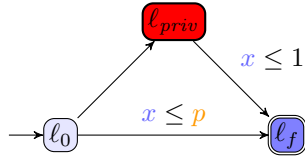
Figure 11: No monotonicity for full timed opacity in L/U-PTAs
