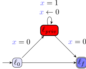
Figure 6: TA for which the set of opaque execution times is \mathbb{N}
