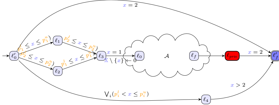
Figure 12: Undecidability of full timed opacity emptiness for L/U-PTAs
