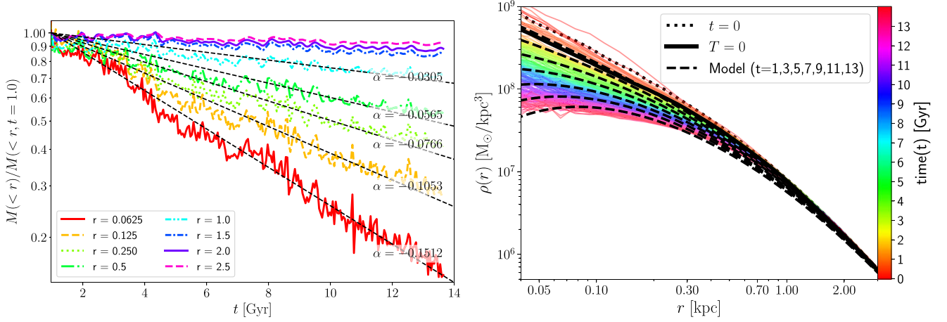
Figure 9. Mass migration and core formation. The left panel shows the ratio between the halo mass within radii r (in kpc) and the corresponding initial mass at T = 0 ( t = t_{\text{diff}} = 1 \text{ Gyr} , as discussed in relation to Fig. 7). The dashed lines are exponential fits, \propto \exp(\alpha T) , with numbers corresponding to \alpha(r) in \text{Gyr}^{-1} . The exponential decay may be derived from a simple theoretical model for the mass transfer; in its context \alpha is predicted to scale with the inverse of an energy relaxation time [obtained using equations (14), (10), and (16)]. The right panel shows the corresponding evolution in density. Theoretical expectations are shown by the dashed lines. They are obtained by differentiating equation (15), starting from an NFW fit to the dark matter density in the simulation at T = 0 . To reduce uncertainties arising from fluctuations in the density profile around T = 0 , we average simulation outputs over the range 0.5 \text{ Gyr} \leq t \leq 1.5 \text{ Gyr} (as in Fig. 7). Model predictions are shown at T = 0 (fitting the averaged profile), and at 2, 4, 6, 8, 10, and 12 Gyr, corresponding to times 1, 3, 5, 7, 9, 11, and 13 Gyr.
