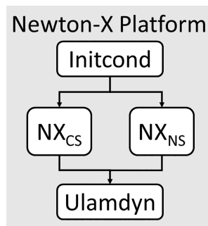
Figure 1. Newton-X platform. Newton-X is branched into four stand-alone programs: Initcond for nuclear ensembles, spectra, and initial conditions; Newton-X CS and NS for dynamics; and Ulamdyn for data analysis, including unsupervised ML.
