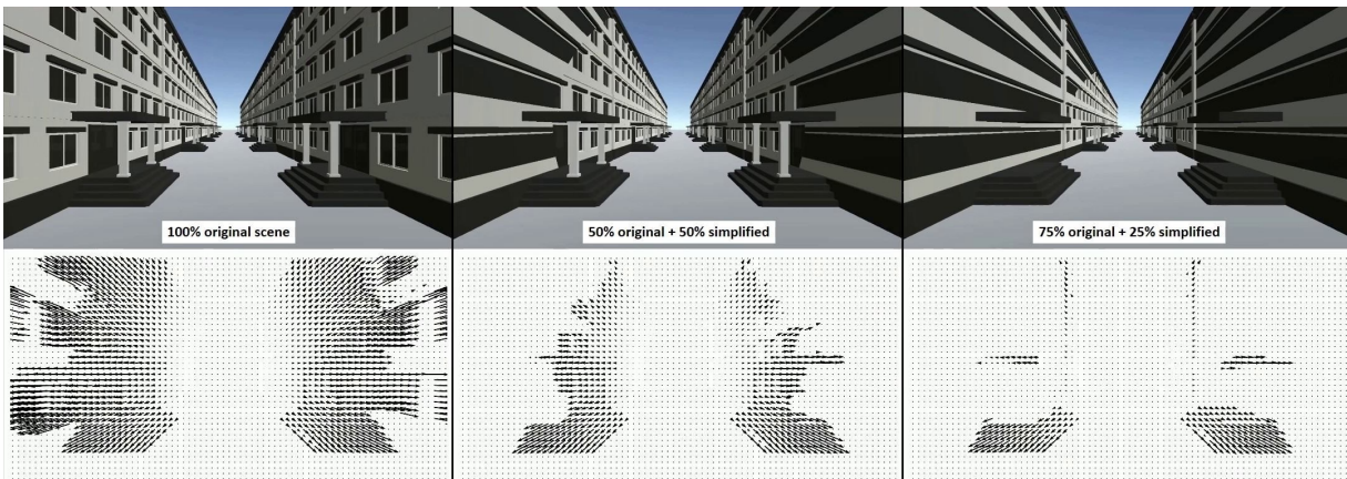
Figure 1: Simplification of the scene (top) for reducing the optic flow in peripheral FOV (bottom).
