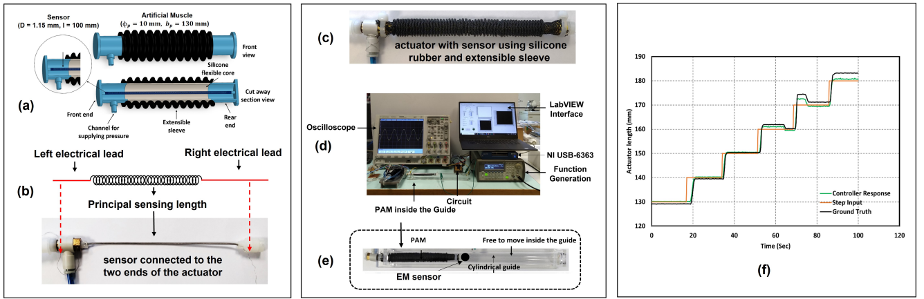
Fig. 6. (a) CAD design of PAM with different components; (b) sensor configuration; (c) sensor integration with the soft actuator; (d) different parts of P-controller; (e) PAM inside the guide; (f) comparison of the lengths estimated from the sensor with the ground truth values during position control.
