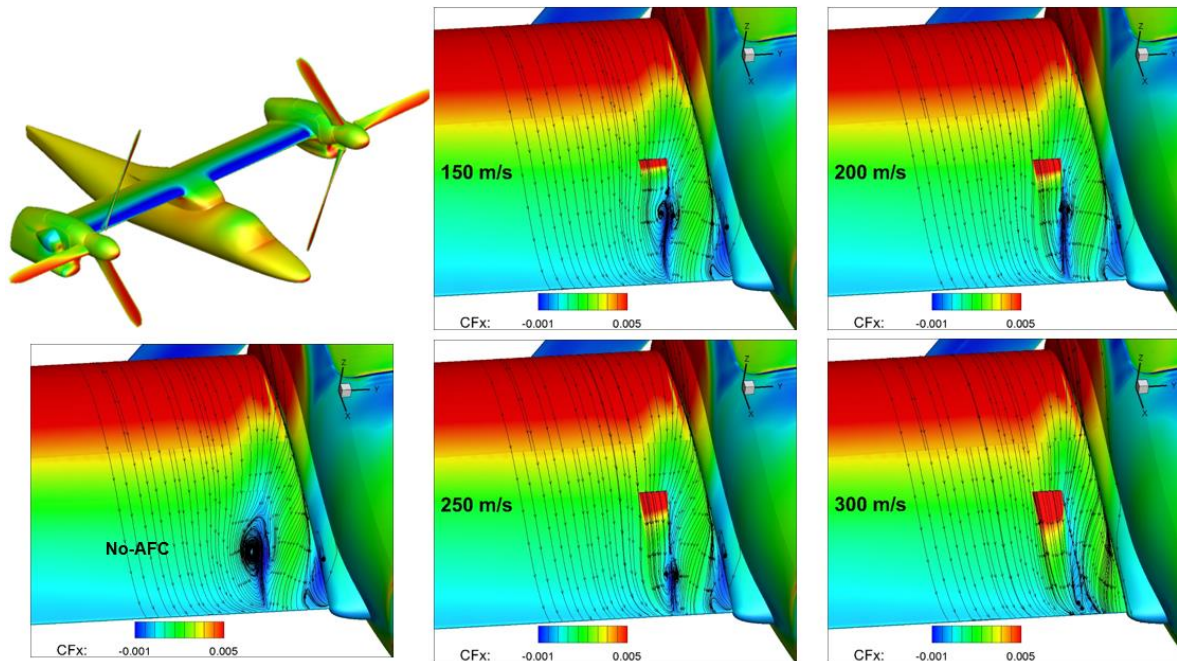
Figure 7: Steady jet control using different jet velocities in the location of the wing-nacelle junction.
