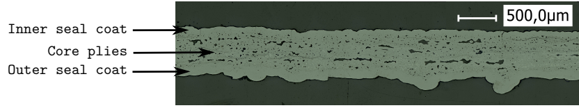
Figure 4: Digital microscopy of the manufactured SiC/SiC cross-section along its axis of revolution cut.
