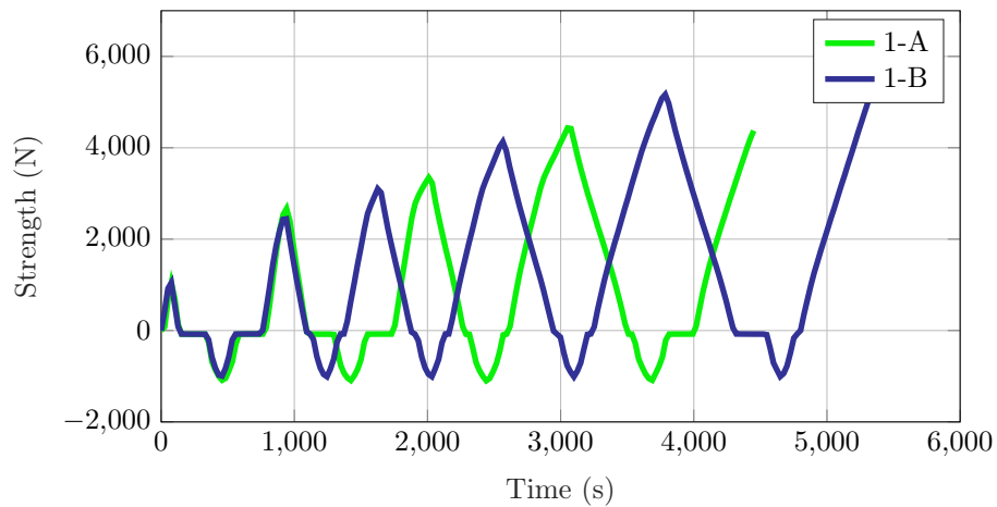
Figure 8: Evolution of the strength as a function of time for each family.
