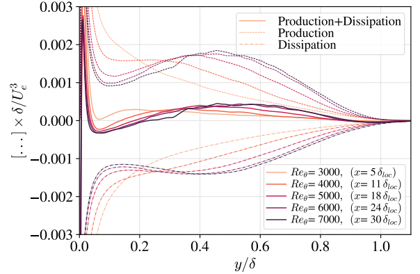
Figure 5. Production and turbulent dissipation rate of turbulent kinetic energy in outer scaling at several streamwise positions.
