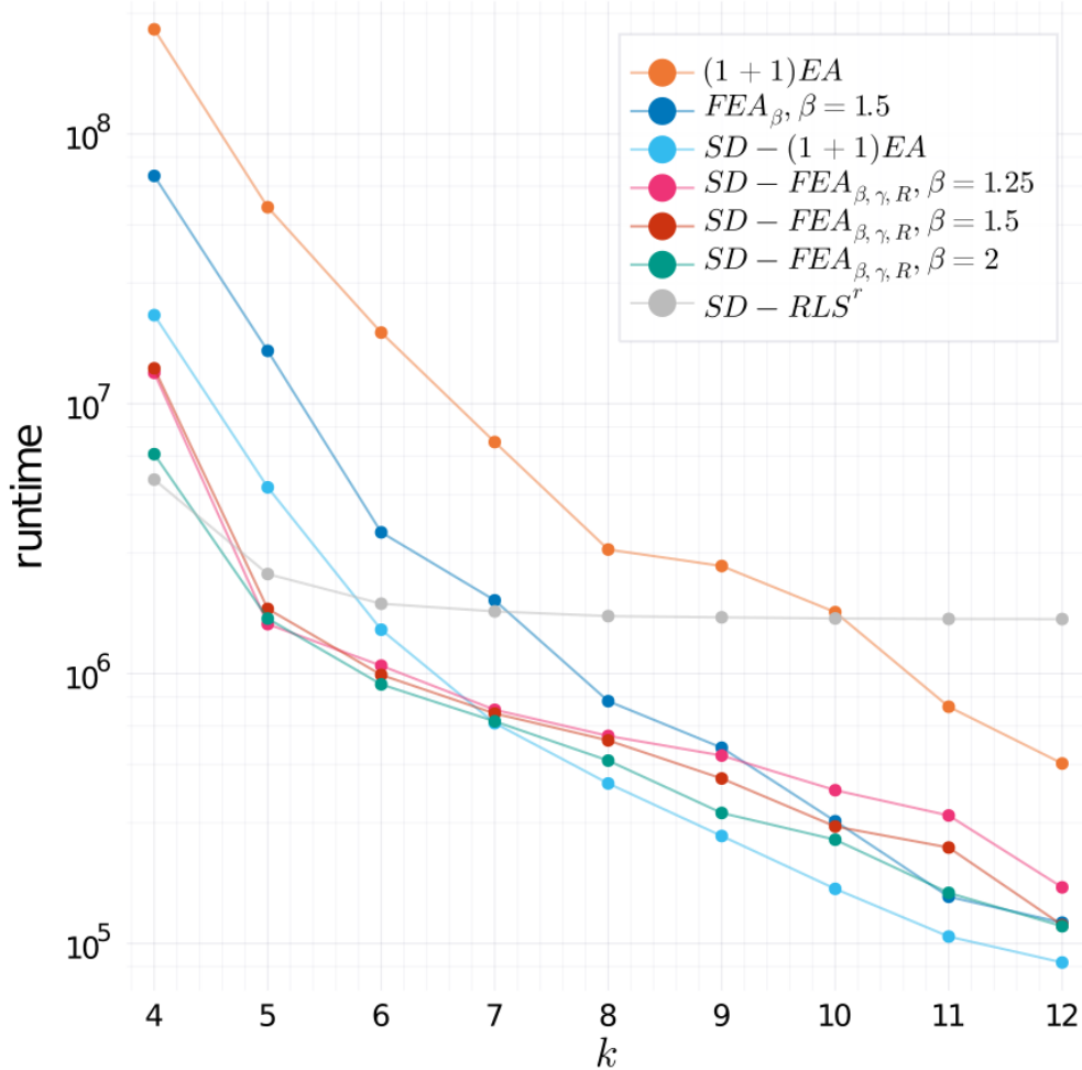
Figure 2: Average number (over 200 runs) of fitness calls the mentioned algorithms spent to optimize \text{JUMP}_{k,4} with different values for k .
