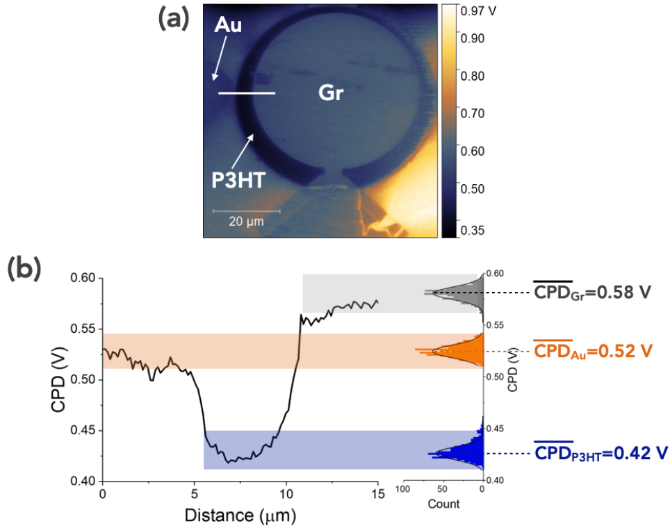
Figure S9. (a) CPD image of a 50 μm device with the different parts (bottom Au electrode, P3HT film and top graphene electrode) indicated. (b) CPD profile along the white line shown in (a) and histograms of the CPD values measured on Au, Gr and P3HT. The black lines are the fits with a Gaussian distribution, the mean CPD values are given in the figure (FWHM of 14 meV in all cases).
