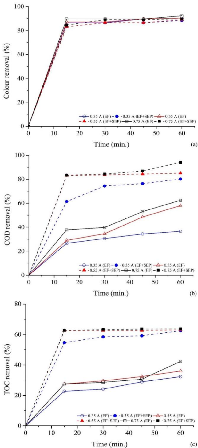
Fig. 3. Effects of time and current on (a) colour, (b) COD and (c) TOC removal by EF and EF/adsorption processes.
