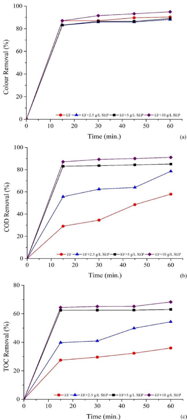
Fig. 7. Effects of time and sepiolite dose on (a) colour, (b) COD and (c) TOC removals by EF/adsorption processes.
