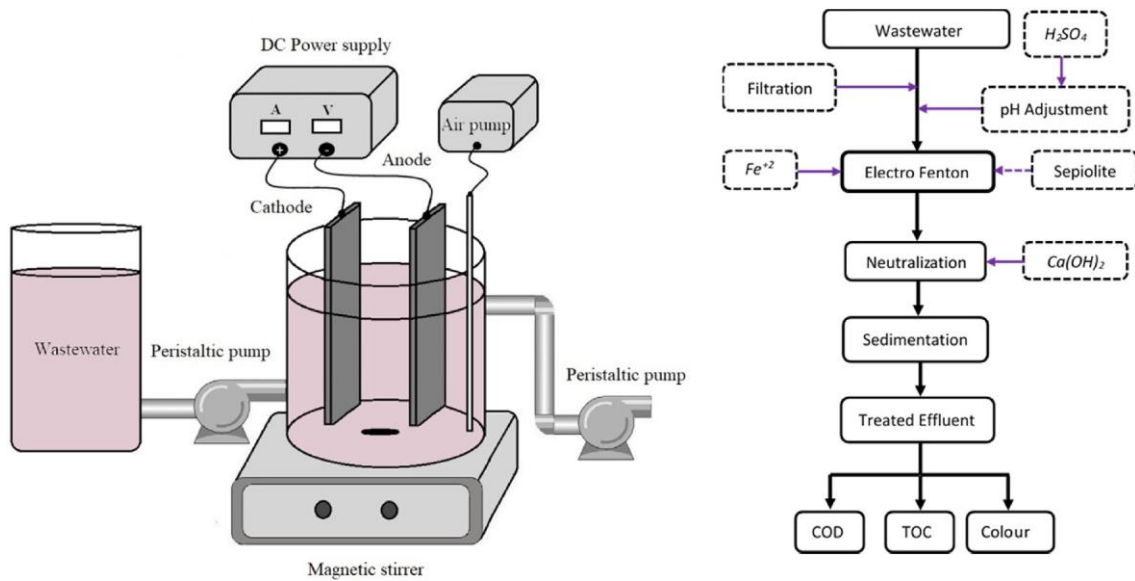
Fig. 1. Schematic diagram of EF reactor and experimental methodology.
