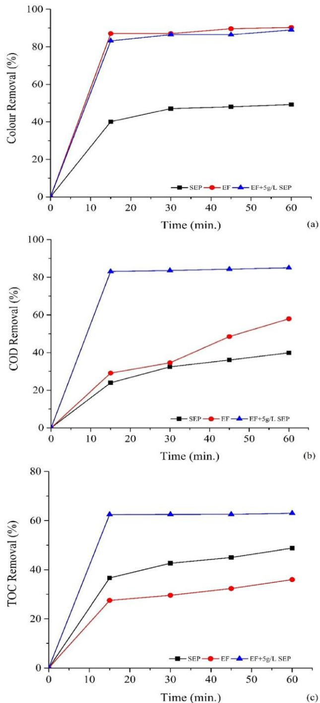
Fig. 8. Comparison of EF, adsorption and EF/adsorption processes for (a) colour, (b) COD and (c) TOC removals.
