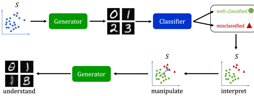
Figure 1: An illustration of the approach. Starting from the latent space S of StyleGAN, we generate a population of images. The images are classified and the information on classification success is added in the space S , where we find the dimensions discriminating well-classified vs. mis-classified images. These dimensions can then be used to visually render the corresponding influential attributes.
