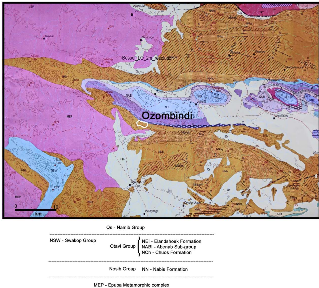
Figure 3. Geological substrate of the Ozombindi calc-tufa and calcrete complex (outlined in white). Base map is an extract from the 1 : 250,000 map sheet, Swartbooisdrif, Sheet 1712. The cascade tufas overlie rocks of the Nosib and Otavi groups.
