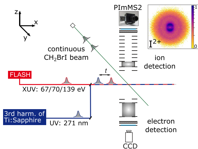
Figure 1. Schematic overview of the experimental setup. A continuous molecular beam of \text{CH}_2\text{BrI} molecules (along y -axis) is intersected by UV and XUV laser pulses (along x -axis) with a controllable delay t . The momentum distributions of ions and electrons are recorded in a double-sided velocity-map imaging (VMI) spectrometer (aligned along the z -axis). An exemplary velocity-map image in the top-right corner shows \text{I}^{2+} ions formed in the UV-pump XUV-probe fragmentation. The spatial overlap of UV and XUV beams was optimized on the ratio of the UV photo-fragments in the image center (indicative of UV dissociation) with respect to the XUV-fragmentation products in the outer feature (created by XUV ionization).
