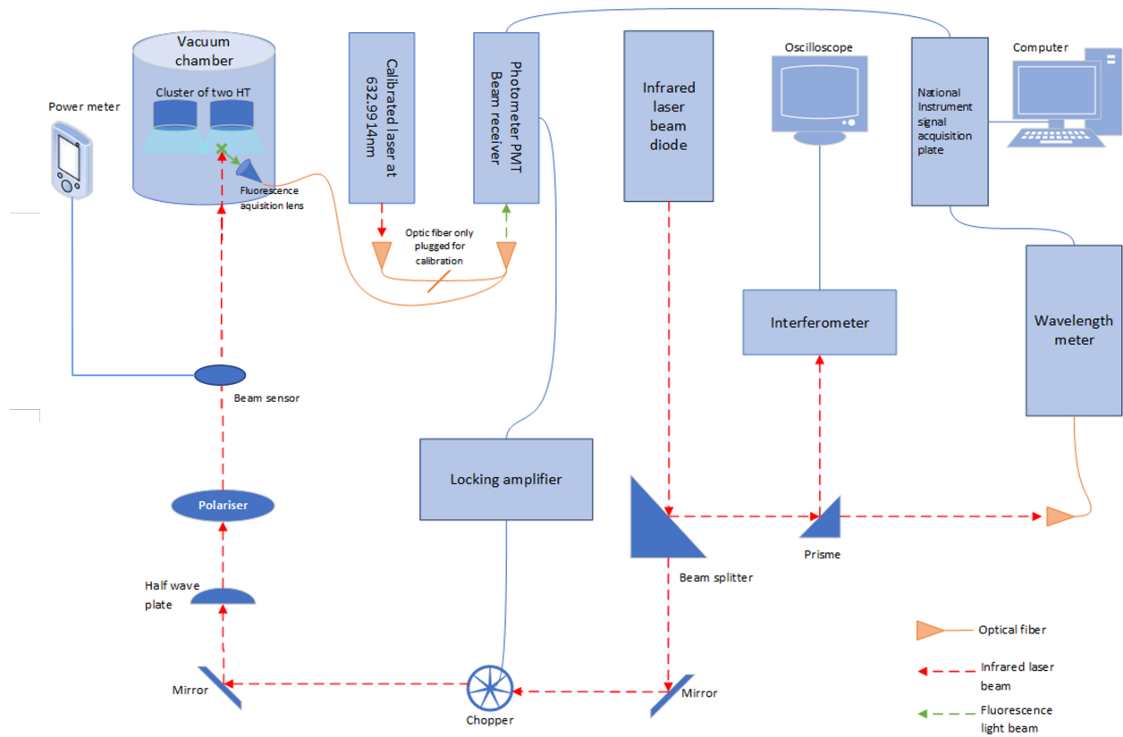
Fig. 3 LIF set up schematic
