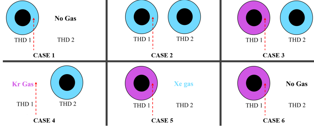
Fig. 6 Various cluster configurations. LIF on Xe^+ ions is solely performed along the axis of THD 1 at x = 20 mm.
