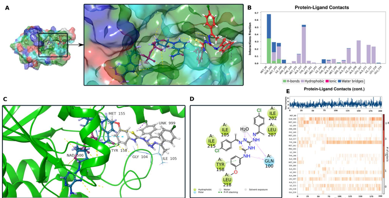
Fig. 8. (A) Representation of BI-16 's binding mode at the InhA surface (B) BI-16 ligand interaction diagram based on 200 ns molecular dynamics simulations. (C) BI-16 binding mode in the InhA active site pocket. The protein is represented by ribbons, whereas the ligand is represented by sticks. (D) MD simulations of 2D ligand interactions with InhA protein amino acid residues. (E) Change of protein–ligand contacts throughout the MD simulations for BI-16 .
