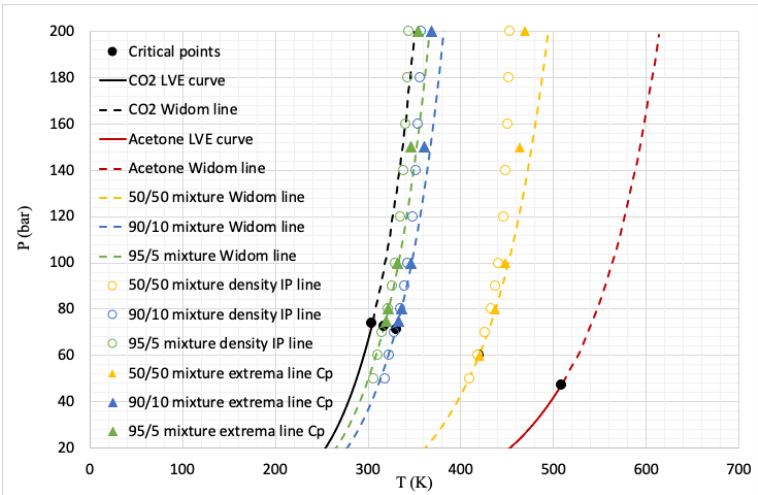
Figure 8: Widom lines, extrema lines and inflexion point lines predicted for the CO 2 /acetone binary mixtures.
