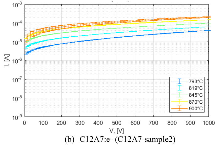
Fig. 14 Raw I-V characteristics (leak current not subtracted) at various sample temperature.
