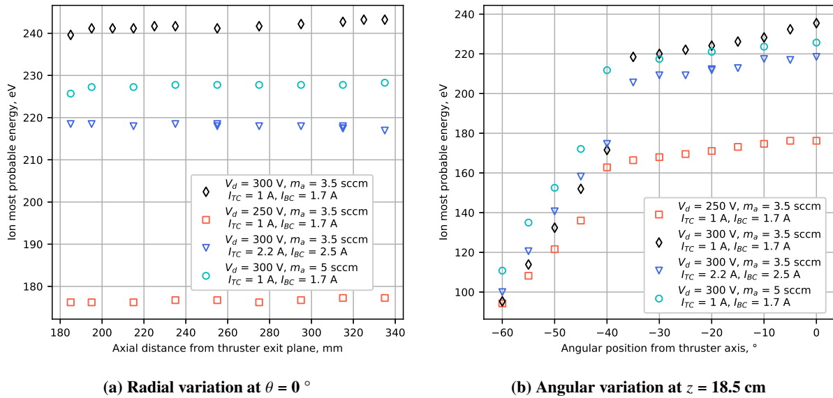
Fig. 9 Spatial variation of the most probable ion energy, for four operating conditions
