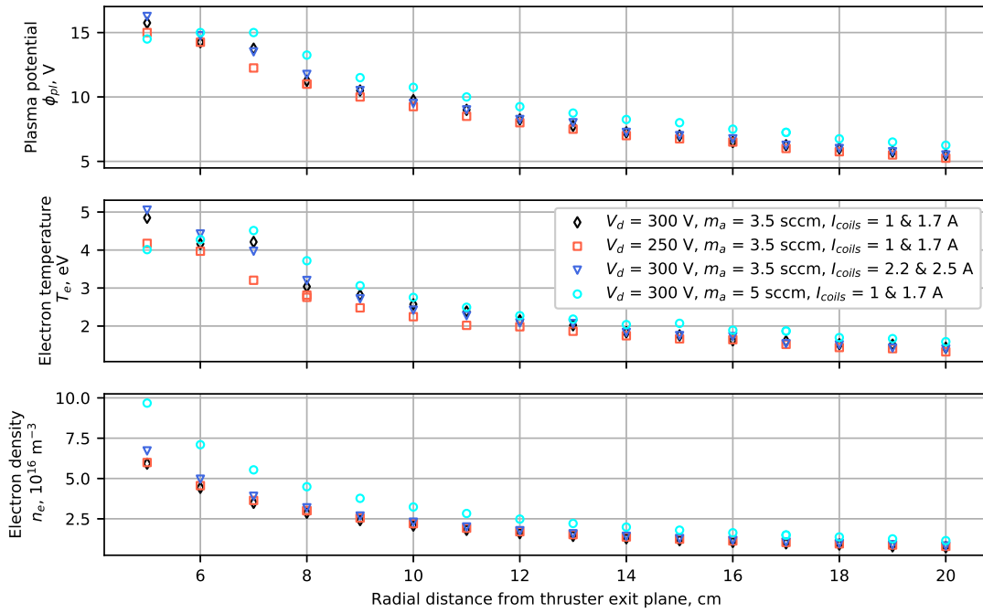
Fig. 6 Variation of plasma properties T_e , n_e and \phi_{pl} along the thruster axis ( \theta = 0^\circ ), for four different operating conditions
