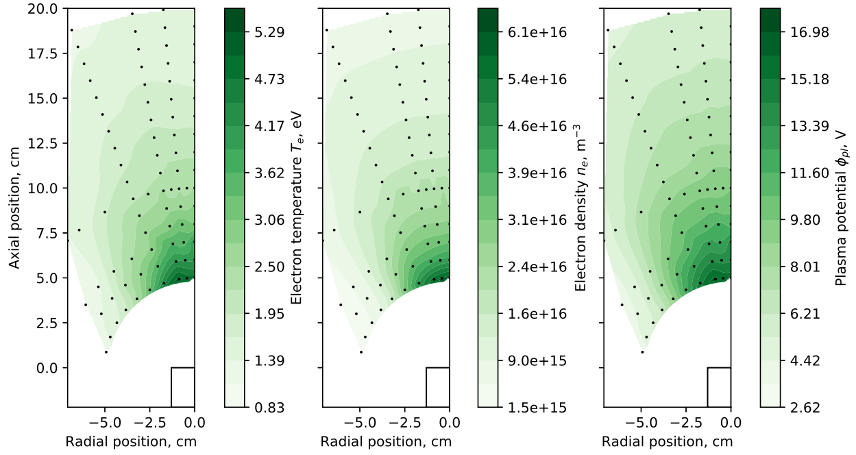
Fig. 5 2D maps of the plasma properties T_e , n_e and \phi_{pl} measured with the LP in the conditions: I_{TC} = 1 A, I_{BC} = 1.7 A, V_d = 300 V, \dot{m}_a = 3.5 sccm
