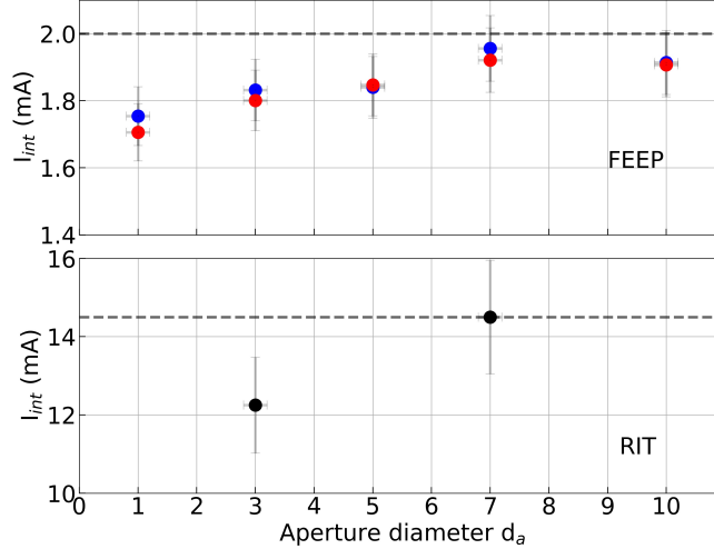
Fig. 6 Evolution of the ion current measured by a FC with different inlet apertures. Top: FEEP thruster firing with 2 mA and 7kV. Bottom: RIT operating at 14.5 mA and 2 kV.
