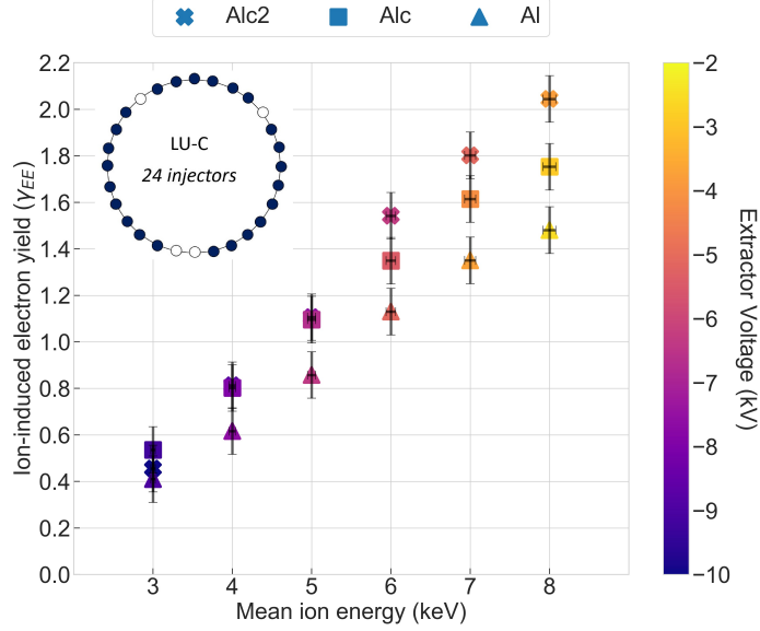
Fig. 8 Ion-induced electron yield obtained for the FEEP with different collector geometries. The thruster fires at 2 mA.
