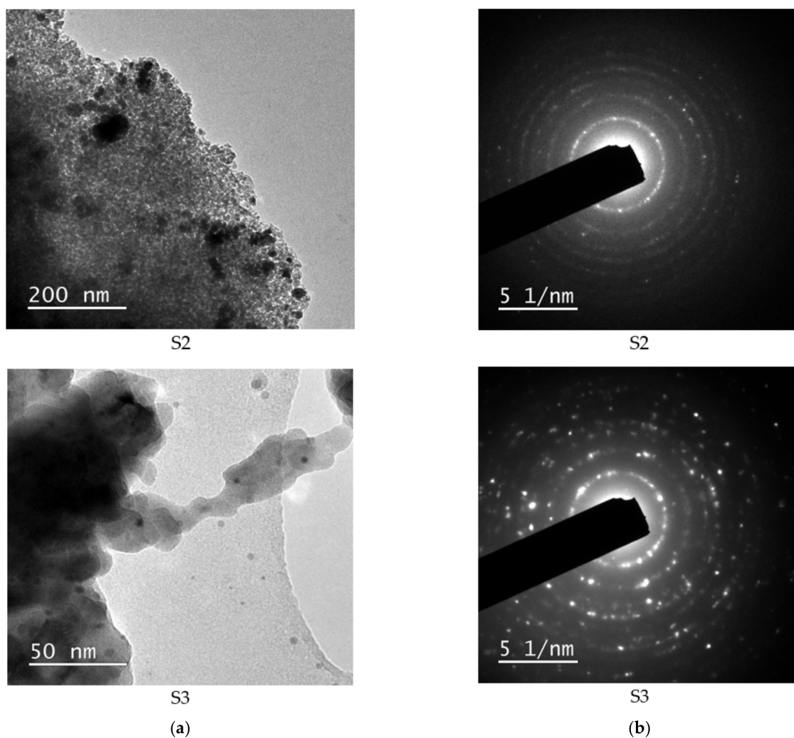
Figure 3. (a) TEM micrographs and (b) SAED images of samples with S2 and S3.
