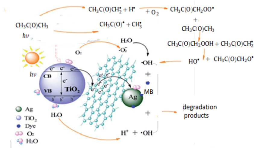
Figure 8. Suggested mechanism of MB photodegradation for the TiO 2 -Ag nanoparticles.
