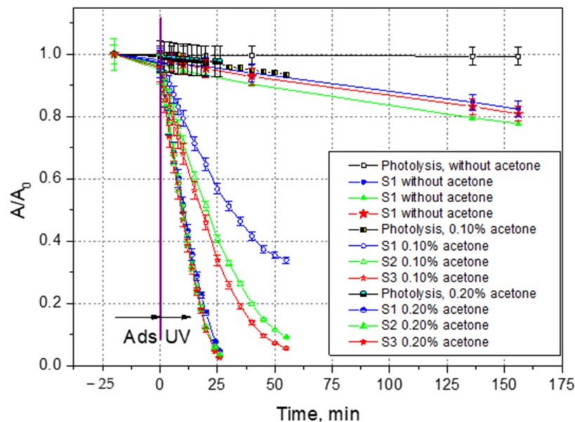
Figure 6. MB removal from the solution by photolysis (blank experiment), photocatalysis in the presence of S1, S2 and S3, and effect of acetone addition in the reaction system (4 ppm MB, 0.03 \text{g L}^{-1} photocatalyst).
