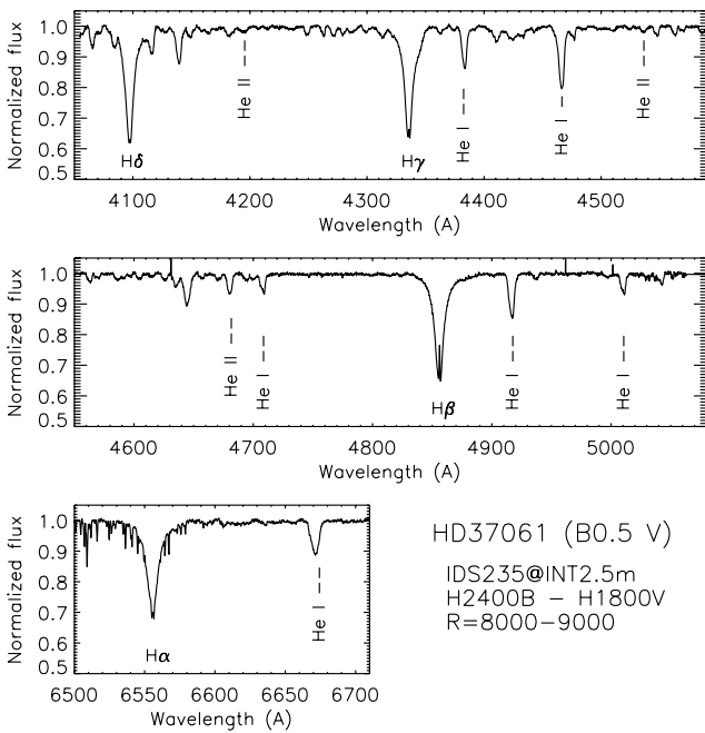
Fig. 3. IDS-INT optical spectrum of HD 37061. The H\ I and He\ I - \Pi lines used for the spectroscopic analysis of the star are indicated.
