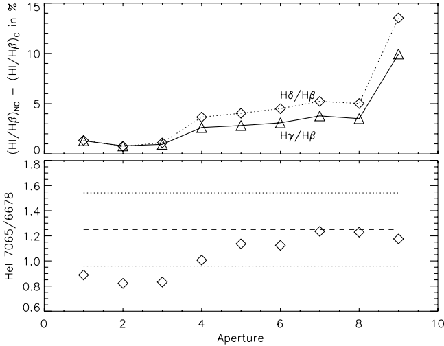
Fig. 9. Upper panel: difference between the non-extinction-corrected H\gamma/H\beta and H\delta/H\beta ratios from the C and NC spectra (see text for explanation). Lower panel: He\ I\ 7065/6678 line ratio from the NC spectra (9 apertures). The mean and standard deviation values corresponding to the bright Huygens region (obtained from data by O’Dell & Harris 2010) are also indicated as a dashed and dotted lines, respectively.
