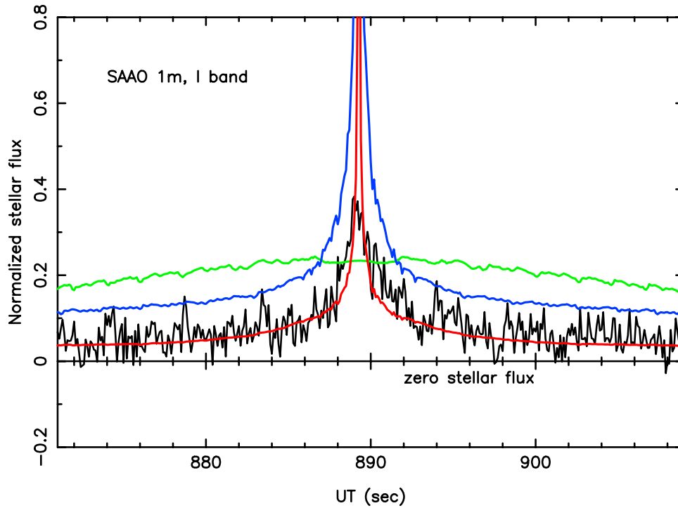
Figure A3. Example of a fit to the SAAO 1-m central flash (black curve). We use here the nominal [Rannou et al., 2004] zonal wind profile multiplied by \eta = 1.10 , and a correction to the impact parameter of \Delta g'' = +5.0 km; see Table 3. The fluxes have been normalized between zero (complete disappearance of the star) and unity (corresponding to the unocculted stellar flux). The green (resp. blue) solid line is the expected flux from the primary (resp. secondary) stellar image, coming from the southern (resp. northern) limb, if the atmosphere were transparent. The small fluctuations observed in the model are caused by the discrete layers (50 m in height) used for calculating the vertical refraction of the stellar rays in Titan's atmosphere; see Appendix A. The red solid line is a linear combination of the primary and secondary fluxes, smoothed by a stellar diameter of 2.2 km projected at Titan. This combination is obtained with a optical depth (along the line of sight) of \tau_{\text{sup}} = 1.1 for titanocentric latitudes \phi \geq \phi_{\text{sup}} = 55^\circ\text{N} and \tau_{\text{inf}} = 2.2 for latitudes \phi \leq \phi_{\text{inf}} = 40^\circ\text{N} . These optical depths have been adjusted so that the derived flash (red curve) has the same area as the data (black curve). The calculated flash is too narrow compared to the data, so that a further smoothing is needed to fit the observations; see Figure A4.
