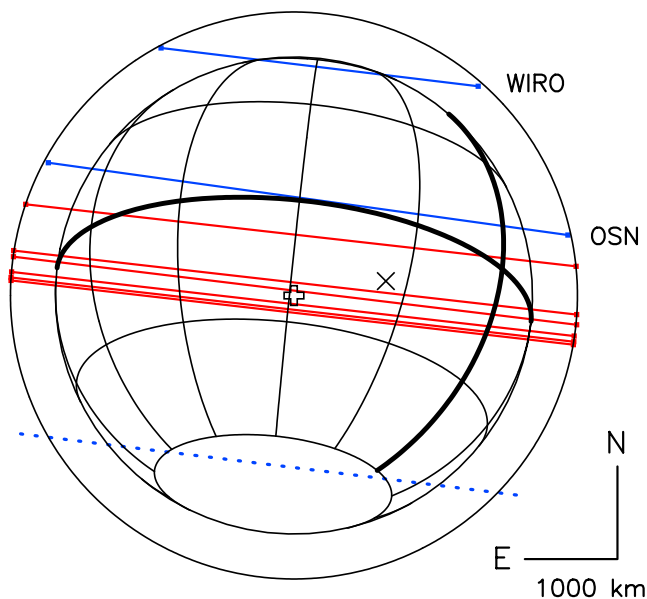
Figure 6. Titan's aspect for the two occultations of 14 November 2003. Celestial J2000 north and east directions and the scale in kilometers are given by the straight segments at the lower right corner. One arcsec corresponds to 6078 km projected at Titan, and the sphere represents the solid surface of a satellite, with a radius of 2575 km. The thick parallel delineates Titan's equator, and the thick meridian represents the anti-Saturn direction (i.e., longitude 180^\circ on Titan). The times symbol ( \times ) gives the expected Titan's center using the DE405 + TASS7.1 Titan ephemeris and the star position of equation (1). This center is the origin of the (f', g') coordinates used in the text. The red lines show the chords observed during the first occultation, using the timings of Table 2. They correspond, from south to north, to SAAO, Cederberg, Gifberg, Maïdo, Sandfontein, and Windhoek (see Figure 7 for an expanded view). The cross marks Titan's center according to a circular fit to the red chords. The Observed-Calculated (O-C) shift between the two centers (times and cross) is 0.163 arcsec toward the east ( \Delta f' = +992 km) and 0.026 arcsec toward the south ( \Delta g' = -155 km). The blue lines are the chords observed at OSN and WIRO, during the second occultation. They have been shifted to lie on the circle defined by the red chords; see text for details. Finally, the dotted line is the chord observed at Mérida, for which no usable light curve could be derived.
