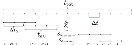
Fig. 4: Schematic of the generation of a statistical ensemble \mathcal{S}(t_{av}, \Delta t_0) of N_{samples} subsets of possible time-averaged signals \mathcal{S}_l .
