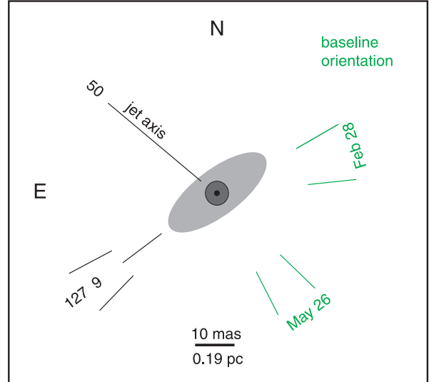
Fig. 8. Sketch of our model for the mid-infrared emission from the inner parsec of Centaurus A. We identify the unresolved point source of <6 \text{ mas} FWHM (dark grey) with the VLBI core ( FWHM = 0.5 \pm 0.1 \text{ mas} , indicated as black dot). It is surrounded by an elongated structure of dust emission (light grey) the major axis of which is orientated along \text{PA} = 127^\circ \pm 9^\circ as inferred from the orthogonal baselines observed on May 26. From the visibilities observed with two baselines on February 28 we derive a major axis length of about 30 mas. Note that the major axis orientation is consistent with being perpendicular to the radio jet axis, and the axis ratio can be explained by a thin disk the axis of which is inclined by \sim 66^\circ with respect to our line-of-sight.
