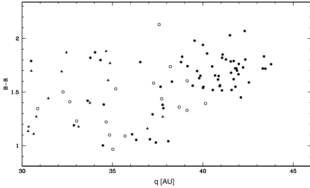
Fig. 7. Color of the KBOs as a function of their perihelion distance q in AU (from Hainaut and Delsanti on-line dataset; Classical KBOs are shown as filled circles, SDOs as open circles, and Plutinos as filled triangles). A lack of blue objects with very large q and a red cluster of classical KBOs at q > 40 AU is clearly displayed.
