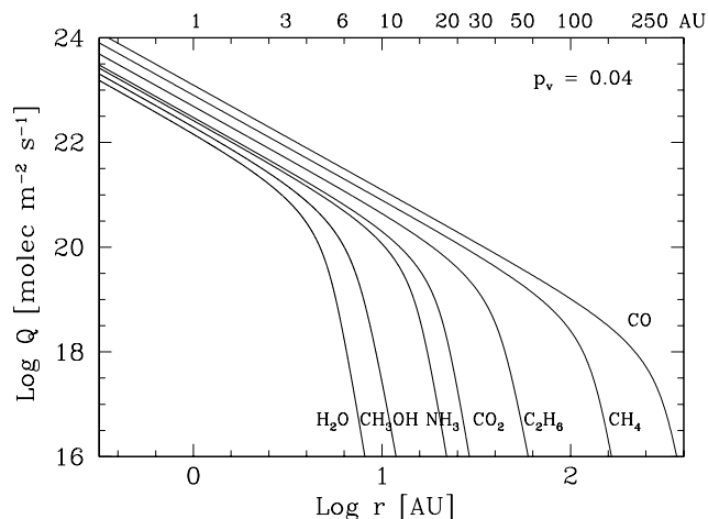
Fig. 4. Sublimation rates of various ices from Meech & Svoren (2004) after Delsemme (1982).
