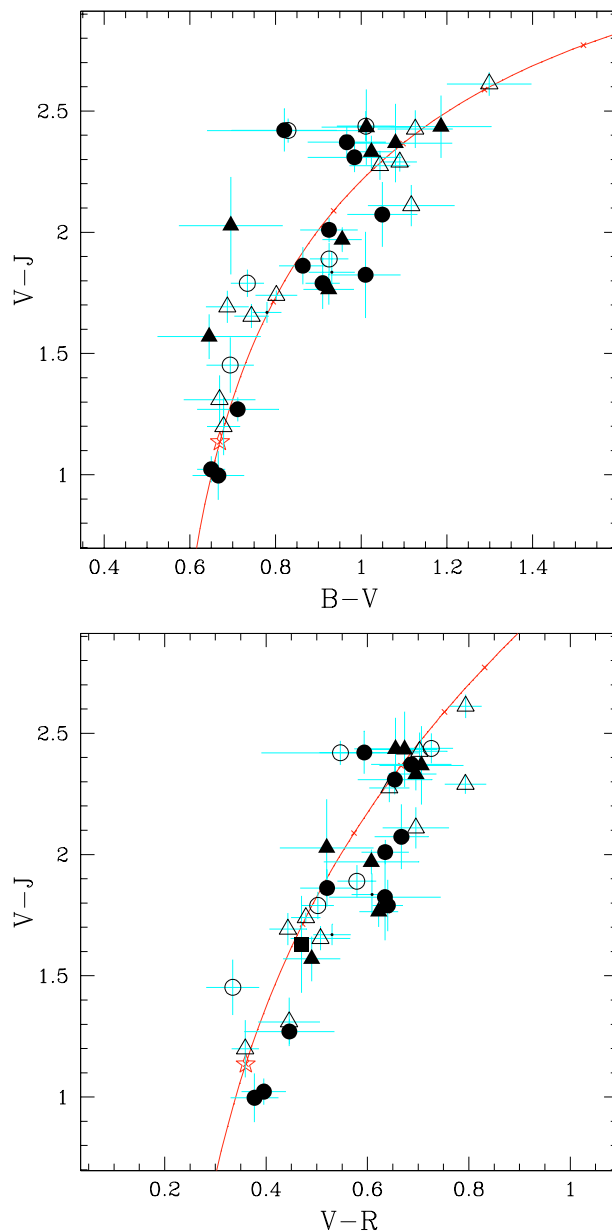
Fig. 2. Color color plots of the averaged colors from the updated version of the compilation presented in Hainaut & Delsanti (2002). The star indicates solar colors. Symbols have the same meaning as in Fig. 1. The thin curve represents the locus of objects with a linear reflectivity spectrum as described in Delsanti et al. (2001). The broad correlation between B - V and V - J mentioned by McBride et al. (2003) is not as obvious in this larger sample. (This figure is available in color in electronic form.)
