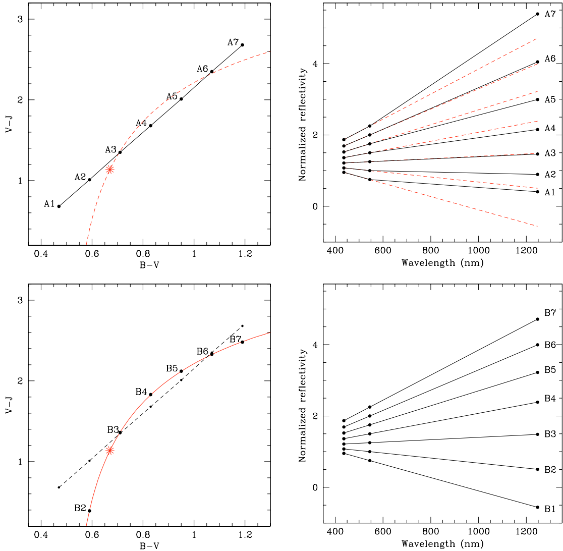
Fig. 3. Left panels are color-color diagrams. The star indicates solar colors. Right panels are the corresponding reflectivity spectra (using Eq. (3), normalized to 1 in the V band and shifted for clarity). Linear color correlations (straight line on top left quadrant) might be useful to derive infrared reflectivities from visible observations. However, they do not imply that objects following such a correlation have a linear reflectivity spectrum (see spectra of objects A1 to A7, top right panel). Perfectly linear spectra (bottom right, objects labeled B1 to B7) correspond in fact to a curve in a color-color diagram (plain curve in bottom left quadrant and dashed curve in top left quadrant). (This figure is available in color in electronic form.)
