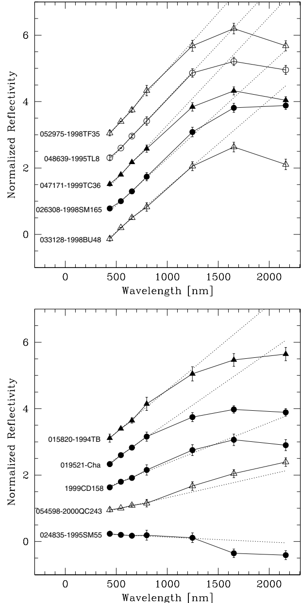
Fig. 1. Normalized reflectivity spectra. Symbols: resonant objects (filled triangles), classical objects (filled circles), centaurs (open triangle), scattered disk objects (open circle). The reflectivities are obtained from the simultaneous BVRIJHK photometry using Eq. (3). The spectra are normalized to 1 at the V filter wavelength and shifted for clarity. The dotted line is a linear fit to the V , R and I reflectivities.
