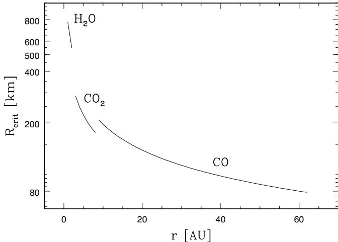
Fig. 5. Variations with the heliocentric distance of the critical radius above which an object is able to keep its bound coma.
