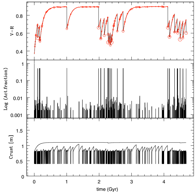
Fig. 6. Evolution of a Plutino on a circular, inclined orbit. The top panel displays the variations of the average color of the object. Collisions are indicated by a circle whose size is logarithmically related to that of the impactor. The second panel shows the fraction of the surface on which ice sublimation occurs, and the third one the minimum and maximum thickness of the crust over the surface of the object. (This figure is available in color in electronic form.)
