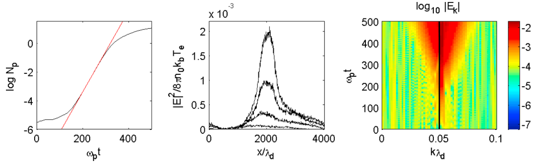
Figure 4. Linear stage of a beam plasma instability (same beam parameters as in Figure 2) in the presence of a gaussian density cavity characterized by \delta n_{\max}/n_0 = -0.03 and \sigma_{\delta_n} = 200\lambda_d . (left) The logarithm of the number of plasmons as a function of time. The straight line is a linear fit with a slope \gamma = 0.03\omega_p . (middle) The electrostatic energy density profile at four different times ( \omega_p t = 250, 300, 350 , and 400 from bottom to top) at the end of the linear phase. (right) The evolution in time of the wave spectrum (logarithmic scale) during the linear stage, on which the resonant wave vector k = \omega_p/v_b is overlotted.
