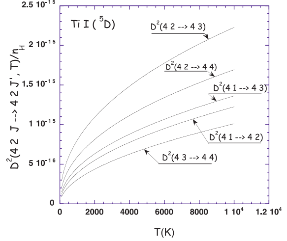
Fig. 4. Polarization transfer rates per unit H-atom density for the upper level of the multiplet 145, D^k(4 2 J \rightarrow 4 2 J', T)/n_H , as a function of T . The rates are given in \text{rad m}^3 \text{s}^{-1} .
