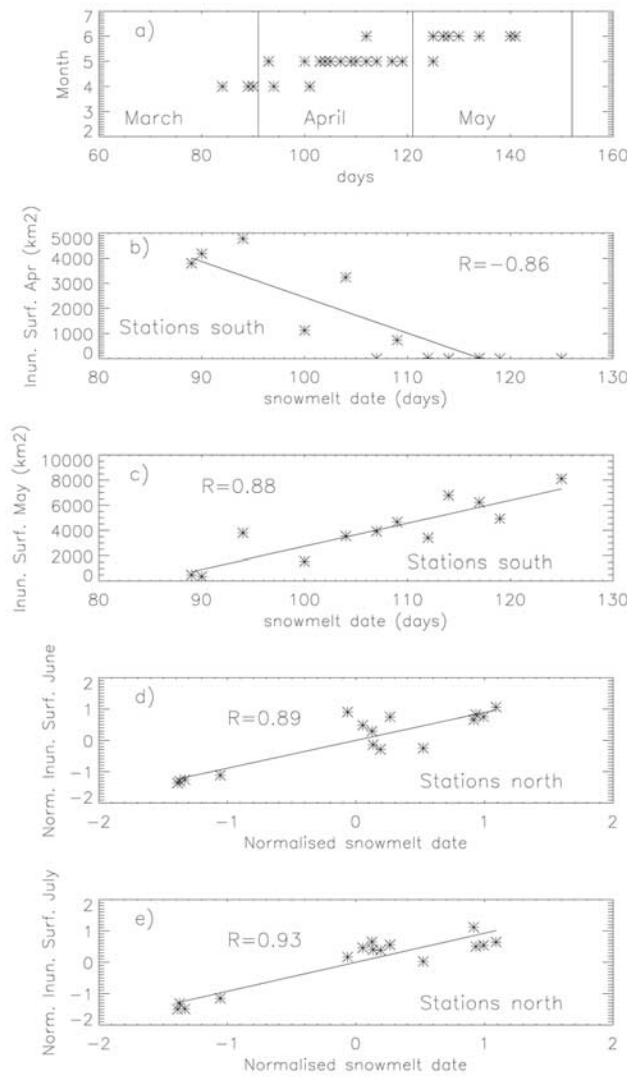
Figure 4. Scatterplot and linear regression results of the in situ snowmelt date observations and the satellite-derived inundated surfaces calculated over a 1^\circ \times 1^\circ area centered on each station during the 1993–1996 period (a) the snowmelt date versus the month of inundated surfaces at maximum for the 7 stations (b) and (c) the snowmelt date versus the inundated surfaces in April and May for the southern stations (stations 5, 6, 7) (d) and (e) the normalized (the mean is subtracted and the resulting values are divided by the standard deviation over the period) snowmelt date versus the normalized inundated surfaces in June and July for the northern stations (stations 1, 2, 3, 4).
