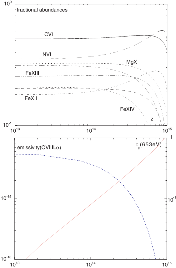
Fig. 4. Fractional abundances of several ions able to absorb the O VIII L\alpha photons ( top panel ), and emissivity of the O VIII L\alpha line and optical thickness in the continuum at the position of the line ( bottom panel ), as functions of the position in the slab, for Model 5 (column density 10^{22} \text{ cm}^{-2} , \xi = 10 , no turbulent velocity).
