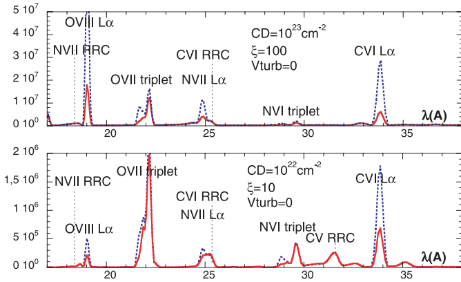
Fig. 5. Reflected spectrum for two models: solid red line: transfer; dashed blue line: escape probability. The ordinate is proportional to F_{\lambda} in photon number (actually it is equal to \nu F_{\nu} ). The spectra are displayed with a spectral resolution of R = 30 .
