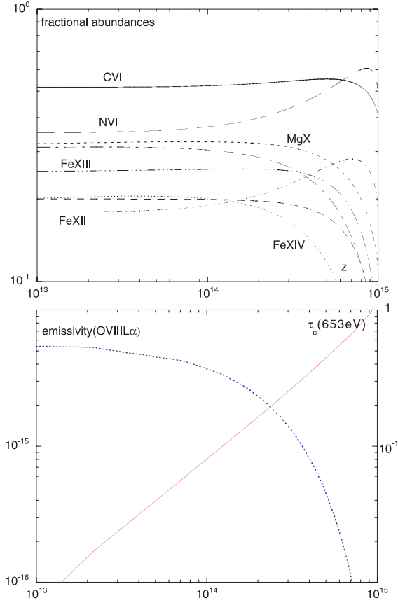
Fig. 4. Fractional abundances of several ions able to absorb the O VIII Lα photons ( top panel ), and emissivity of the O VIII Lα line and optical thickness in the continuum at the position of the line ( bottom panel ), as functions of the position in the slab, for Model 5 (column density 10^{22} \text{ cm}^{-2} , \xi = 10 , no turbulent velocity).
