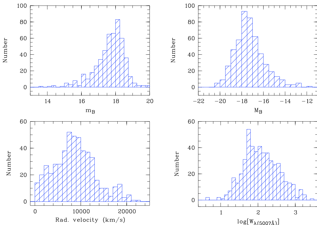
Fig. 1. Distributions of the BCG sample in the zone of HSS of a) total B -magnitude, b) absolute B -magnitude, c) radial velocity and d) equivalent width of [O III 5007] line.
